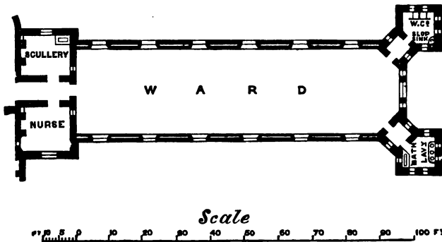
Fig. 1. —WARD AND WARD OFFICES.
